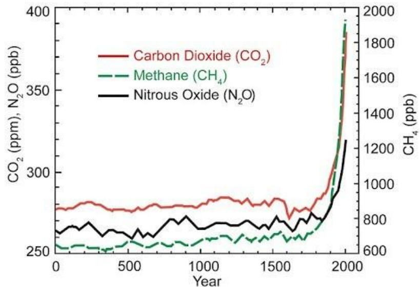
Figure 5. https://archive.epa.gov/epa/climate-change-science/causes-climate-change.html
